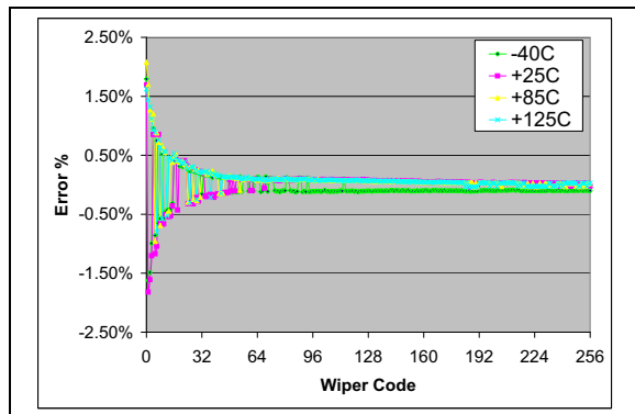
FIGURE 2-15: 5\text{ k}\Omega – Worst Case R_{BW} from Average R_{BW} ( R_{BW0} – R_{BW3} ) Error (%) vs. Wiper Setting and Temperature ( V_{DD} = 5.5\text{V} , I_W = 190\text{ }\mu\text{A} ).
