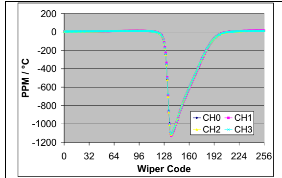
FIGURE 2-80: 100 kΩ – R_{WB} PPM/°C vs. Wiper Setting. ( R_{BW(\text{code}=n, 125^\circ\text{C})} - R_{BW(\text{code}=n, -40^\circ\text{C})} / R_{BW(\text{code}=256, 25^\circ\text{C}) / 165^\circ\text{C}} * 1,000,000 ) ( V_{DD} = 3.0\text{V} , I_W = 24\text{ }\mu\text{A} ).
