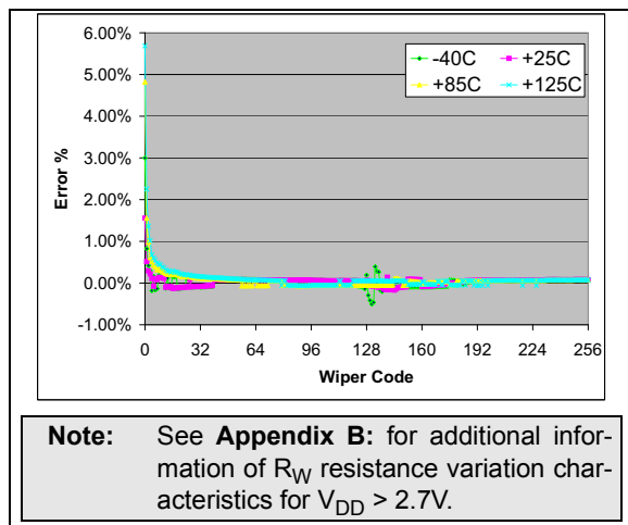
FIGURE 2-78: 100 kΩ – Worst Case R_{BW} from Average R_{BW} ( R_{BW0} - R_{BW3} ) Error (%) vs. Wiper Setting and Temperature ( V_{DD} = 1.8\text{V} , I_W = 15\text{ }\mu\text{A} ).
