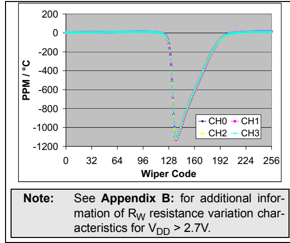
FIGURE 2-81: 100 kΩ – R_{WB} PPM/ ^\circ\text{C} vs. Wiper Setting. ( R_{BW(\text{code}=n, 125^\circ\text{C})} - R_{BW(\text{code}=n, -40^\circ\text{C})} / R_{BW(\text{code}=256, 25^\circ\text{C})} / 165^\circ\text{C} * 1,000,000 ) ( V_{DD} = 1.8\text{V} , I_W = 15\text{ }\mu\text{A} ).
