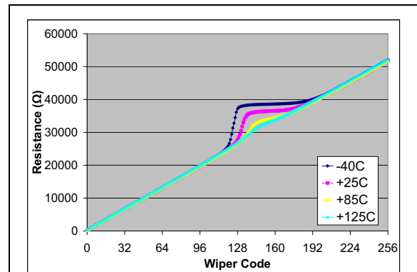
FIGURE 2-54: 50 kΩ – R_{WB} ( \Omega ) vs. Wiper Setting and Ambient Temperature ( V_{DD} = 3.0\text{V} , I_W = 48\text{ }\mu\text{A} ).
