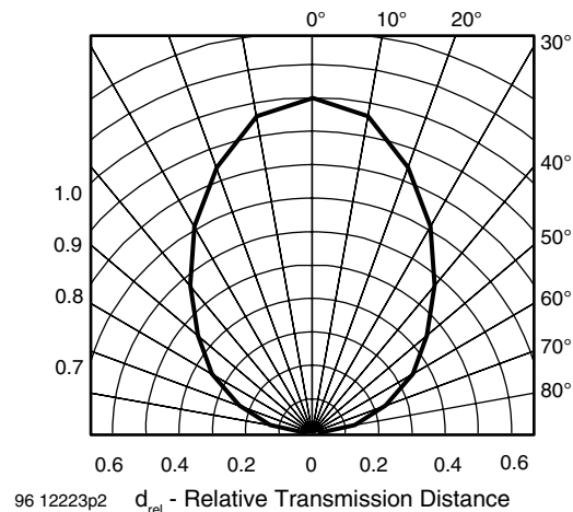
Fig. 12 - Horizontal Directivity
