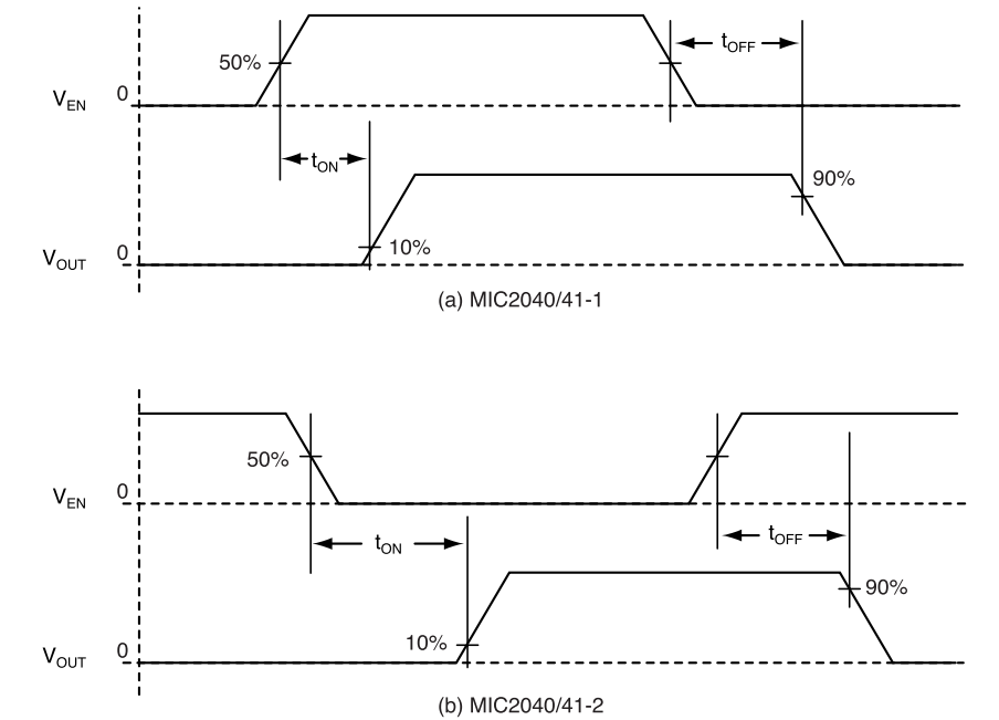
Figure 1. Turn-On/Turn-Off Delay
