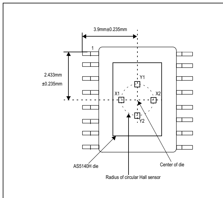
Figure 42: Arrangement of Hall Sensor Array on Chip (Principle)
