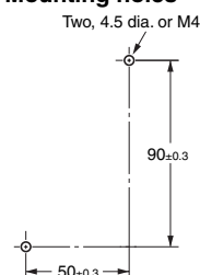
Mounting holes
