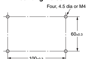
Mounting Holes
