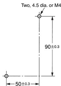
Mounting Holes
