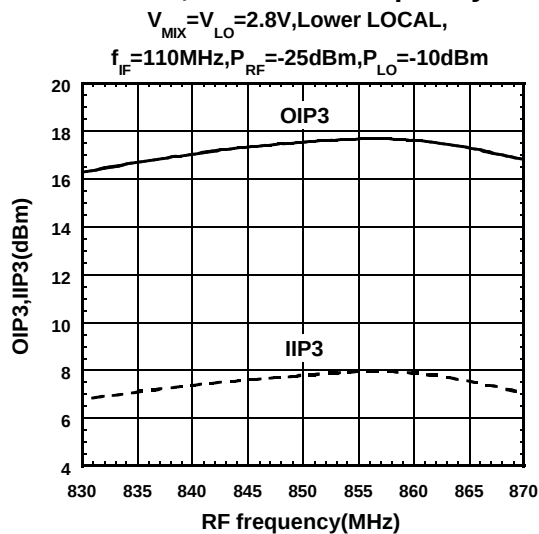
OIP3, IIP3 vs. RF frequency
