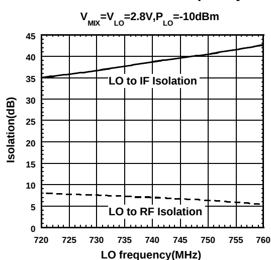
Isolation vs. LO frequency
