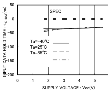
Fig.22 Input Data Hold Time t_{HD:DAT(LOW)}
