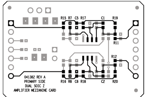
Figure 29. Multiple Feedback Low-Pass Filter 8-Lead SOIC, Dual AMC Configuration
