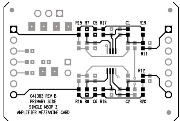
Figure 30. Multiple Feedback, Low-Pass Filter 8-Lead MSOP, Dual AMC Configuration
