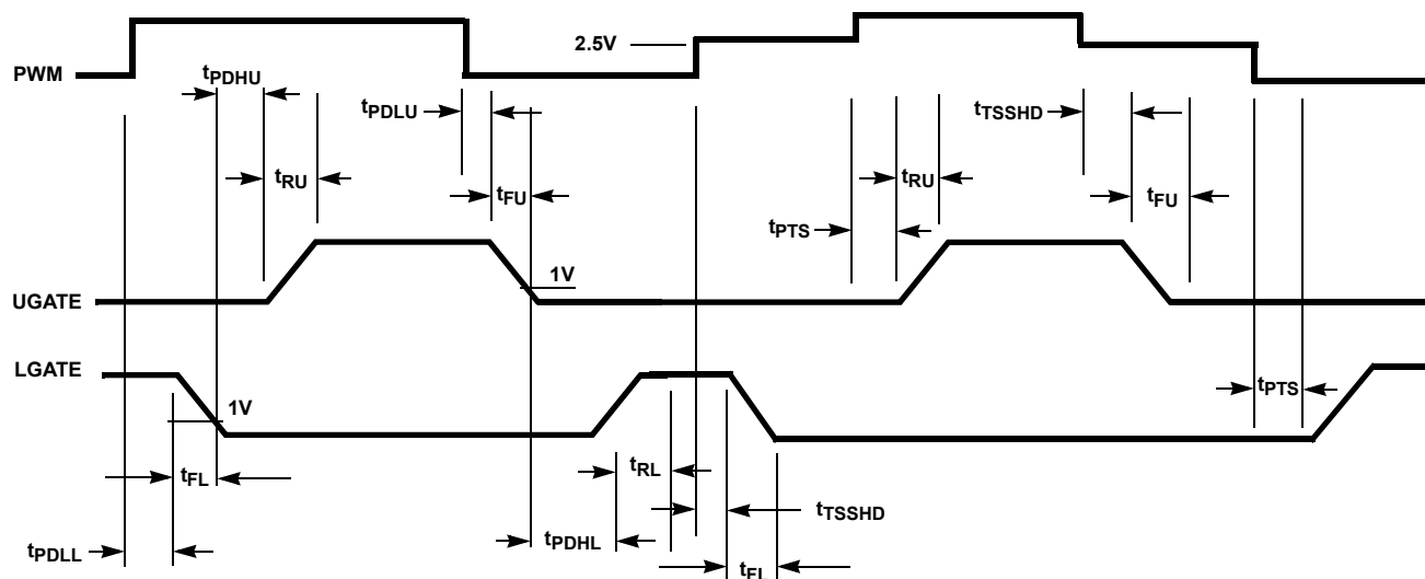
FIGURE 3. TIMING DIAGRAM
