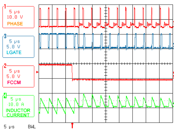
FIGURE 7. CCM TO DCM TRANSITION AT NO LOAD
