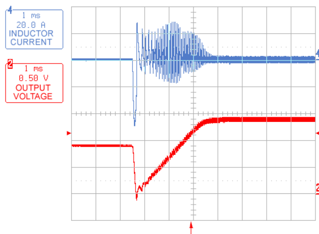
FIGURE 8. PREBIASED START-UP IN CCM MODE
