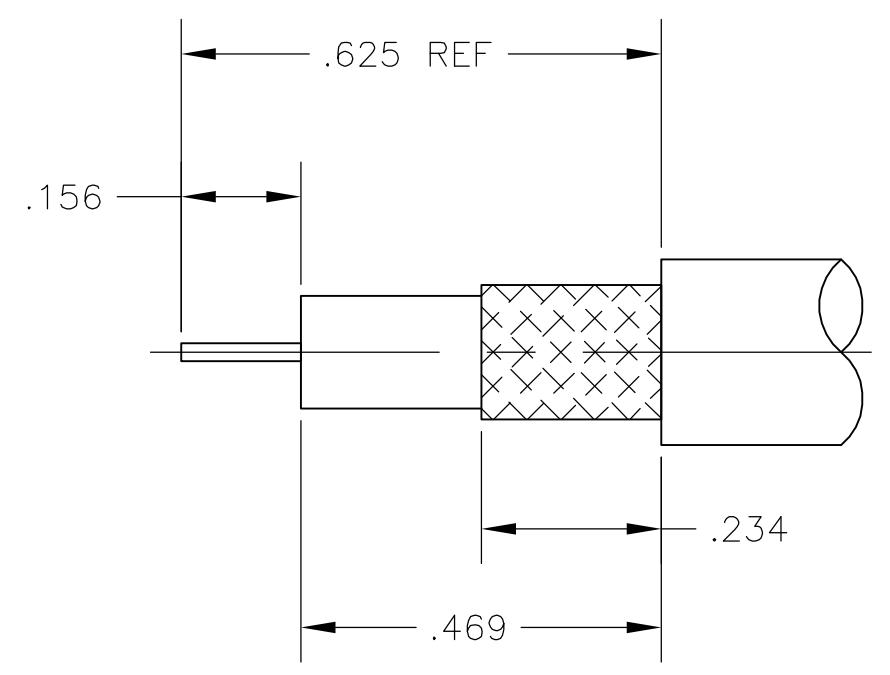
VIEW A
