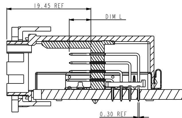
SECTION 1-1 SCALE 2.000
