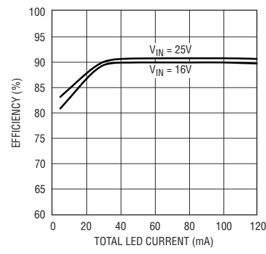
Efficiency vs Total LED Current
