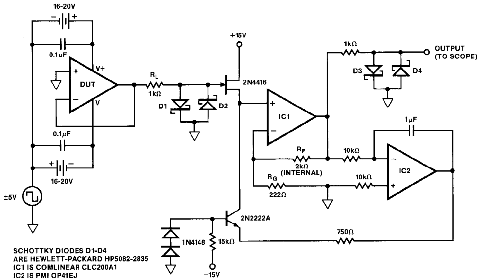
FIGURE 5: OB-42 Settling-Characteristics
