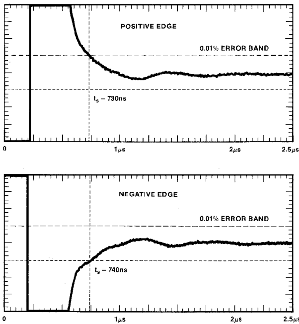
FIGURE 5: OB-42 Settling-Characteristics
