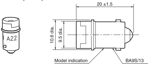
LED A22-6□, 12□, 24□
