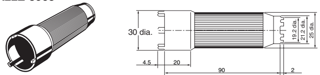
Tightening Tool A22Z-3905
