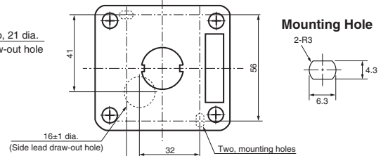
Cable Draw-out Hole (Top View)
