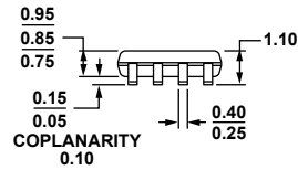
Figure 42. 8-Lead Mini Small Outline Package [MSOP] (RM-8)
