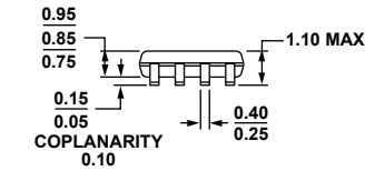
Figure 42. 8-Lead Mini Small Outline Package [MSOP] (RM-8) Dimensions shown in millimeters
