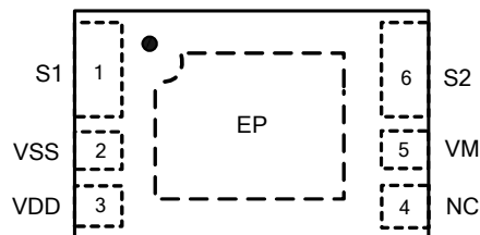
U-DFN2535-6 (Option 2)
