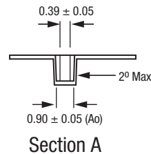
Figure 8. SC-79 Tape and Reel Dimensions
