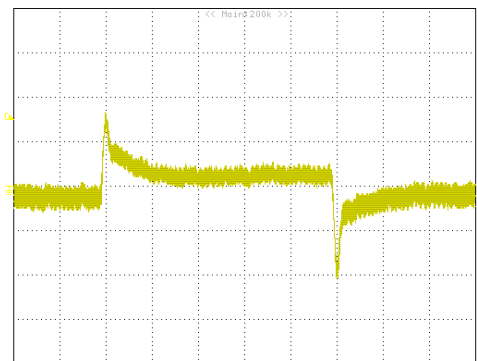
Figure 24: Transient response to dynamic load change at 2.5A/μS from 50%~ 100%~50% of I_o , max at 12Vin, 2.5Vout (Cout = 1uF ceramic, 47uF*2 +10μF ceramic)
