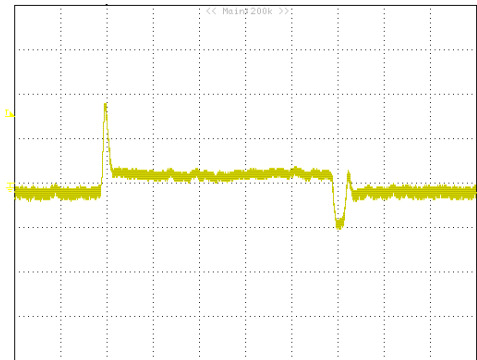
Figure 22: Transient response to dynamic load change at 2.5A/μS from 50%~ 100%~50% of I_o , max at 12Vin, 1.2Vout (Cout = 1uF ceramic, 47uF*2 +10μF ceramic)
