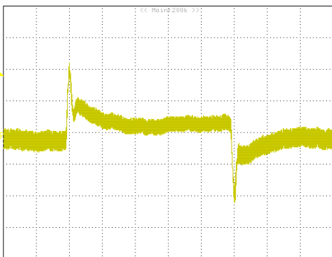
Figure 25: Transient response to dynamic load change at 2.5A/μS from 50%~ 100%~50% of I_o , max at 12Vin, 3.3Vout (Cout = 1uF ceramic, 47uF*2 +10μF ceramic)
