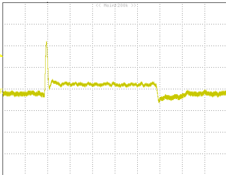
Figure 21: Transient response to dynamic load change at 2.5A/μS from 50%~ 100%~50% of I_o , max at 12Vin, 0.8Vout (Cout = 1uF ceramic, 47uF*2 +10μF ceramic)
