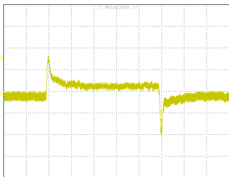
Figure 23: Transient response to dynamic load change at 2.5A/μS from 50%~ 100%~50% of I_o , max at 12Vin, 1.8Vout (Cout = 1uF ceramic, 47uF*2 +10μF ceramic)
