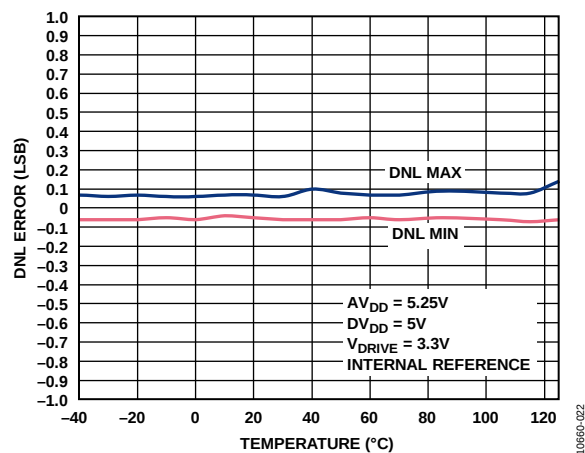
Figure 21. DAC DNL vs. Temperature
