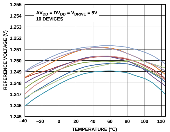
Figure 27. Reference Voltage vs. Temperature
