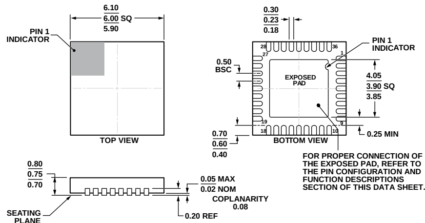
COMPLIANT TO JEDEC STANDARDS MO-220-WJJD. Figure 47. 36-Lead Lead Frame Chip Scale Package [LFCSP_WQ] 6 mm × 6 mm Body, Very Very Thin Quad (CP-36-3) Dimensions shown in millimeters
