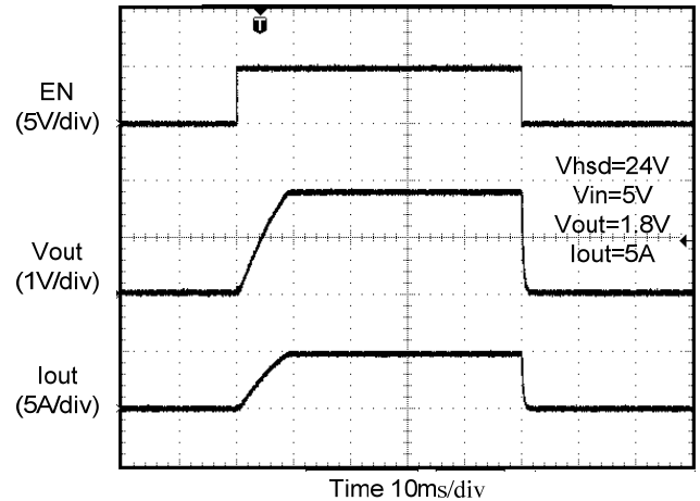
Power-Up/Power-Down
