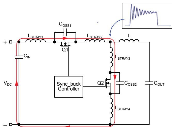
Figure 5. Output Parasitics
