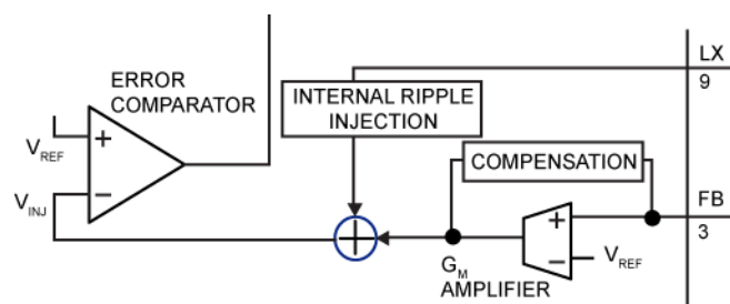
Figure 9. Internal Ripple Injection
