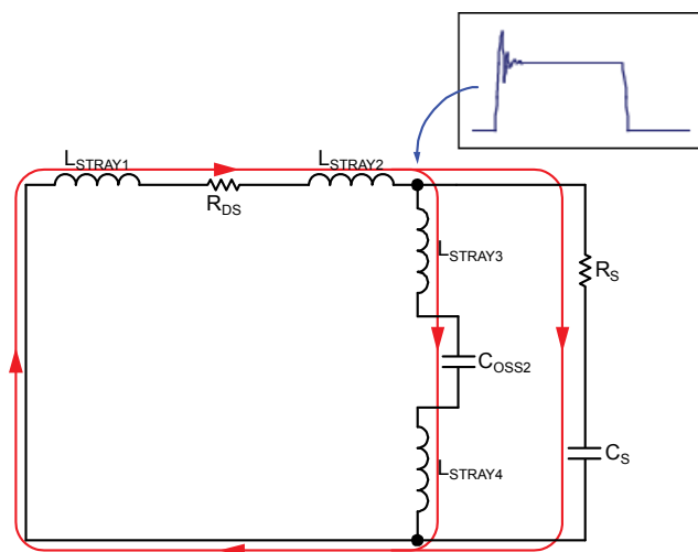
Figure 6. Snubber Circuit
