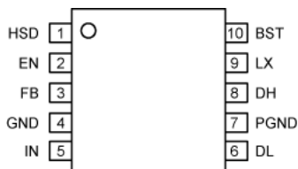
10-Pin MSOP (MM)
