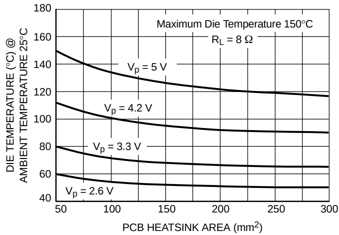
Figure 29. Maximum Die Temperature versus PCB Heatsink Area
