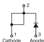
TO-247AC modified
