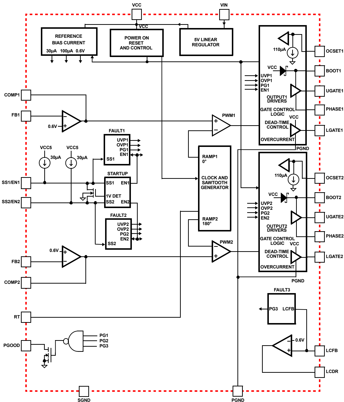
FIGURE 1. BLOCK DIAGRAM
