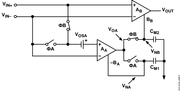
Figure 51. Output Phase of the Amplifier
