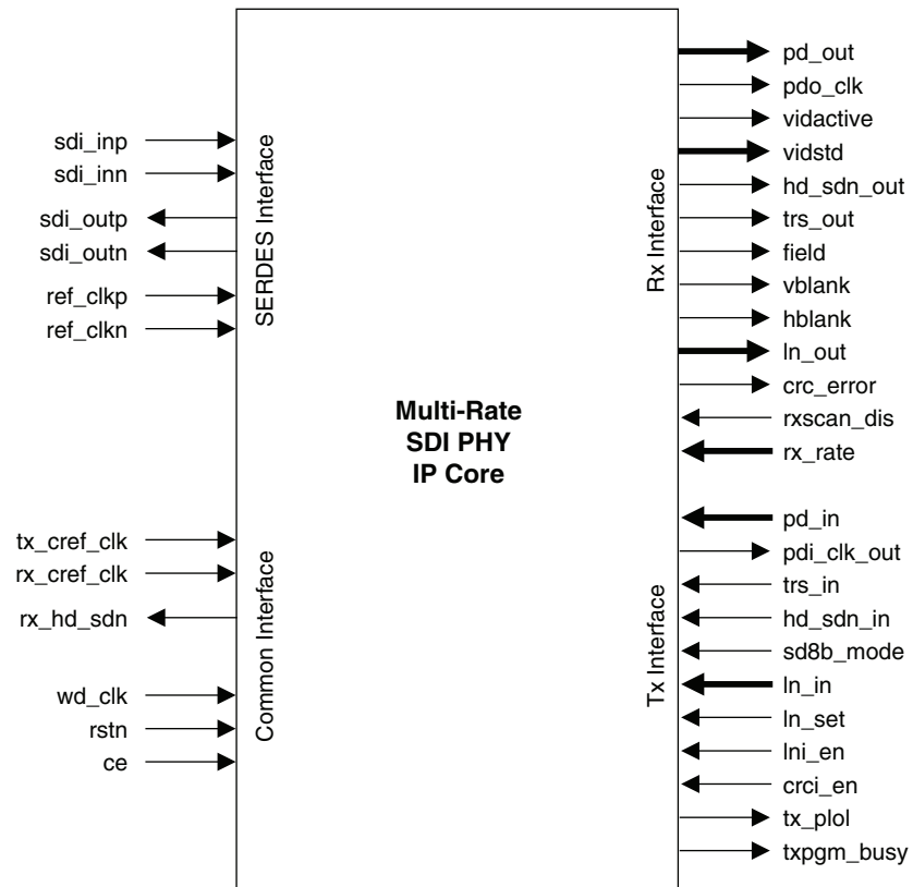
Figure 1. Top-Level Interface for SERDES Inside the IP Core
