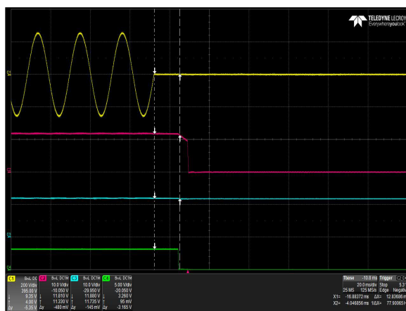
Figure 6: DS1600SPE-3 Hold-up Time – Vin = 264Vac / 47Hz / 0° Full Load: Io = 129.8A, Isb = 3.5A
