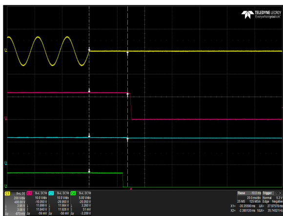
Figure 5: DS1600SPE-3 Hold-up Time – Vin = 90Vac / 63Hz / 0° Full Load: Io = 63.2A, Isb = 3.5A Ch 1: AC Mains Ch 2: Vo Ch 3: Vsb Ch 4: Pwr Good AC Mains V o V sb Pwr Good
