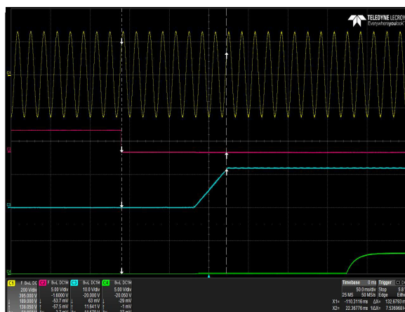
Figure 4: DS1600SPE-3 Turn-on delay via PS_ON_L – Vin = 180Vac Full Load: Io = 129.8A, Isb = 3.5A Ch 1: AC Mains Ch 2: PS ON L Ch 3: Vo Ch 4: Pwr Good
