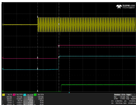
Figure 1: DS1600SPE-3 Turn-on delay via AC mains – Vin = 90Vac Full Load: Io = 63.2A, Isb = 3.5A Ch 1: AC Mains Ch 2: Vsb Ch 3: Vo Ch 4: Pwr Good [Oscilloscope waveform showing turn-on delay]
