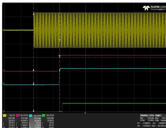
Figure 2: DS1600SPE-3 Turn-on delay via AC mains – Vin = 180Vac Full Load: Io = 129.8A, Isb = 3.5A
