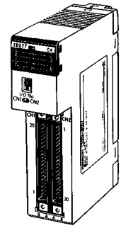
C200H-ID217 (64 DC input pts.)
