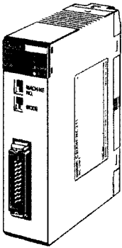
C200H-NC211
