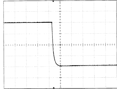
MAX520 NEGATIVE SETTLING TIME
