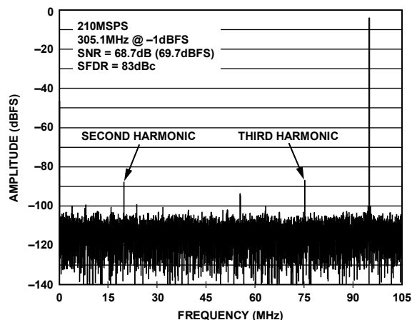
Figure 19. AD9642-210 Single-Tone FFT with f_{IN} = 305.1 MHz
