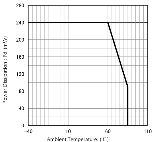
Ambient Temp. vs. Total Value of Power Dissipation
