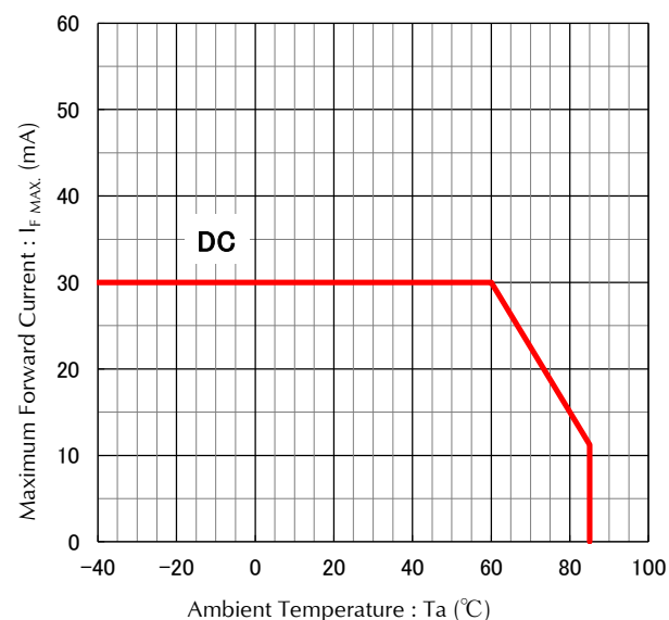
Ambient Temperature vs. Maximum Forward Current 【RED : 3 LED Emitting】
