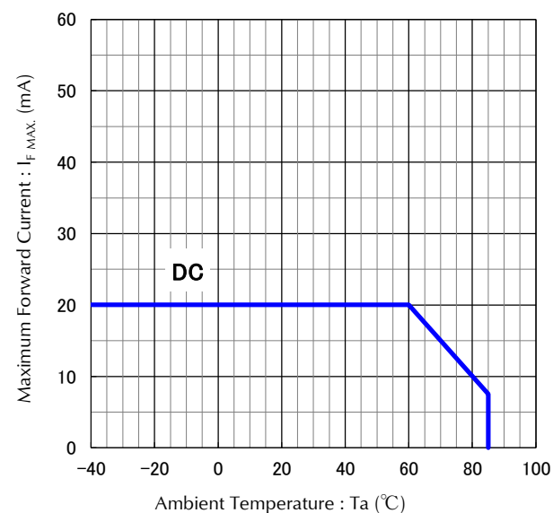
Ambient Temperature vs. Maximum Forward Current 【BLUE : 3 LED Emitting】
