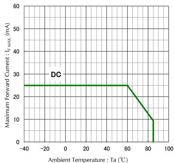
Ambient Temperature vs. Maximum Forward Current 【GREEN : 3 LED Emitting】
