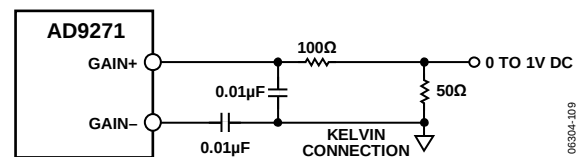
Figure 51. Single-Ended \text{GAIN}_{\pm} Pins Configuration
