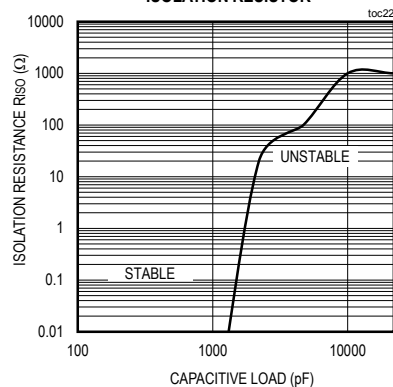
STABILITY vs. CAPACITIVE LOAD AND ISOLATION RESISTOR
