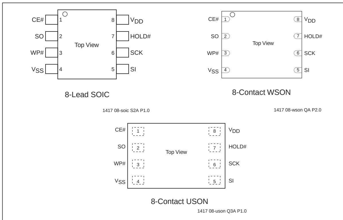
Figure 2: Pin Assignments
