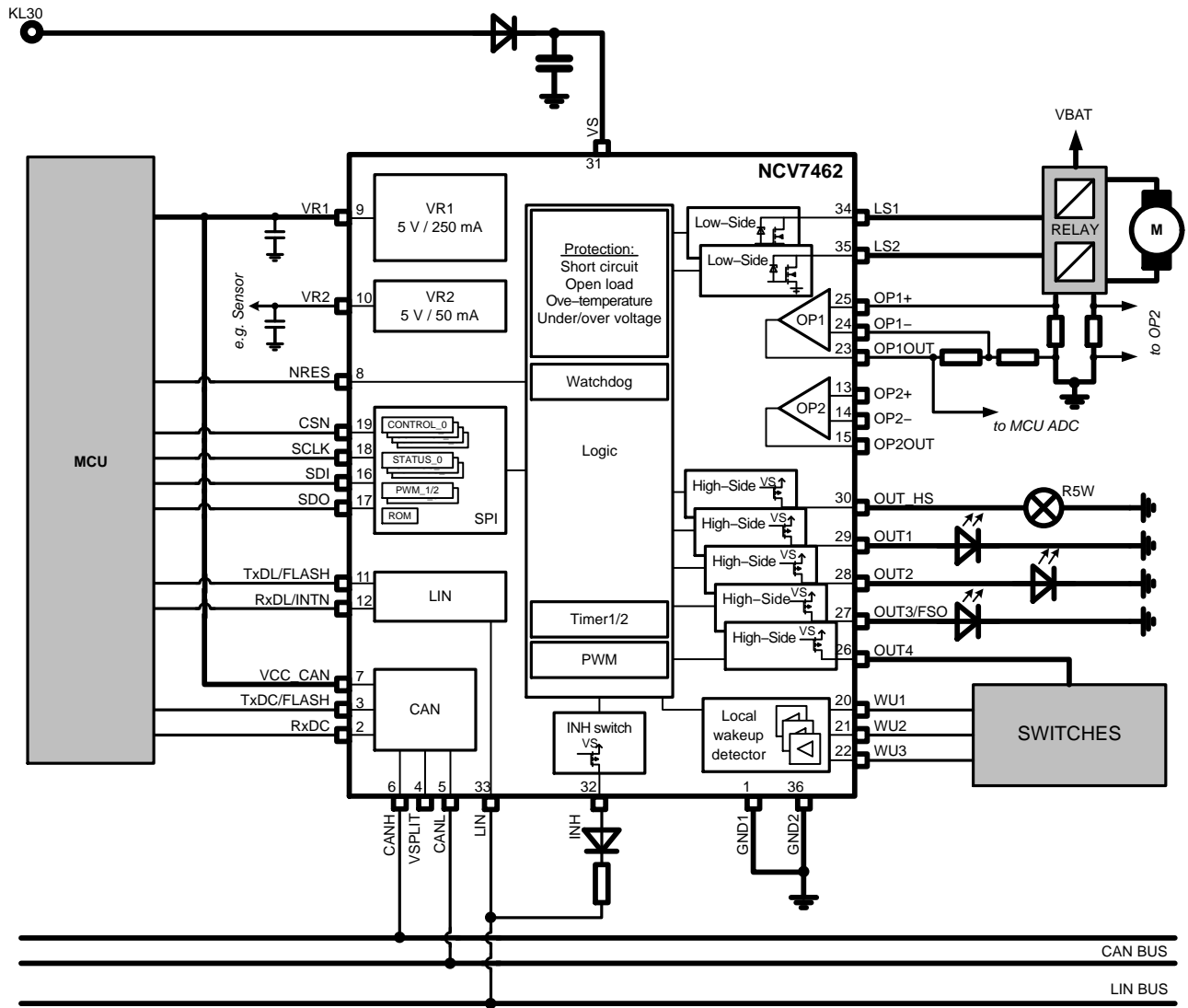
Figure 3. Application Diagram
