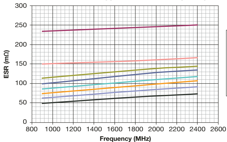
Accu-P® 1210 Typical ESR vs Frequency
