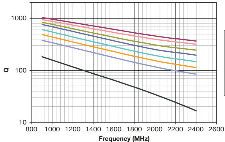
Accu-P® 1210 Typical Q vs Frequency
