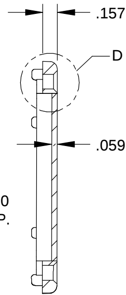
SECTION C-C
