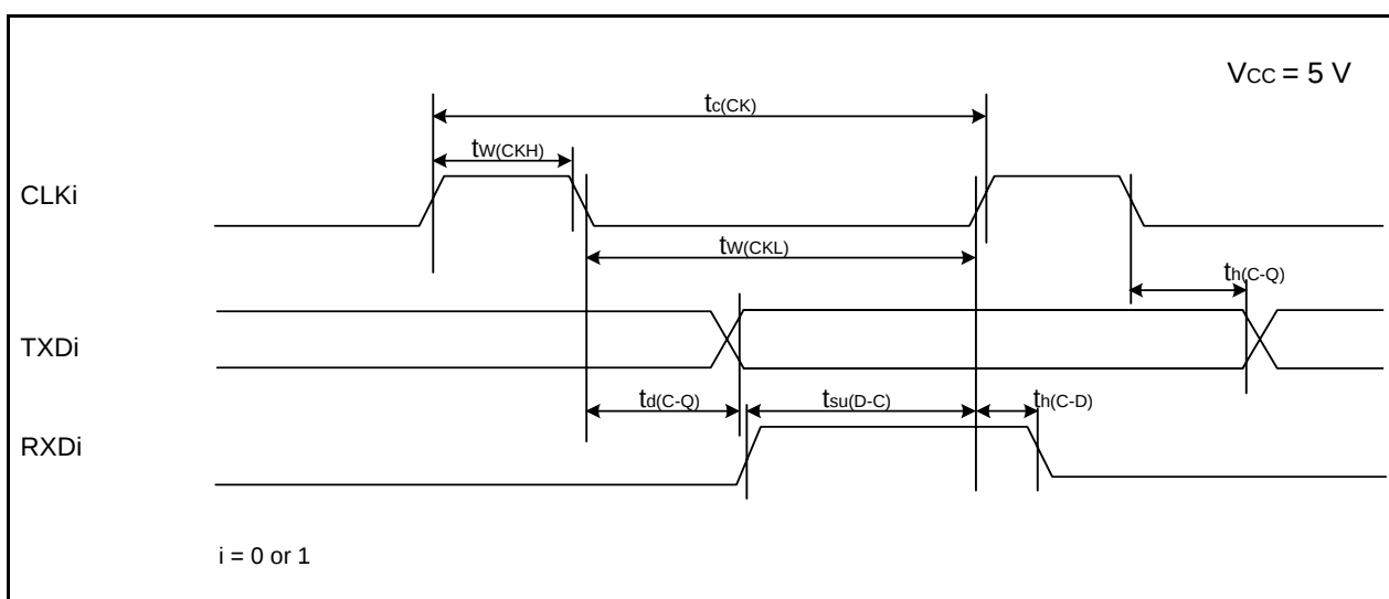
Figure 5.11 Serial Interface Timing Diagram when V CC = 5 V
