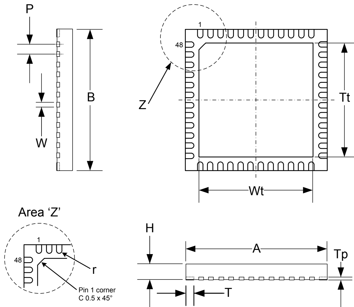
Figure 8.1 QFN(7x7)-48 Package
