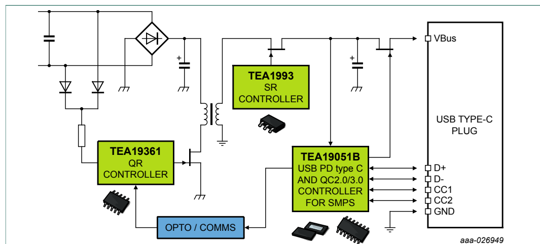
Figure 1. TEA1936xDB1475 principle schematic
