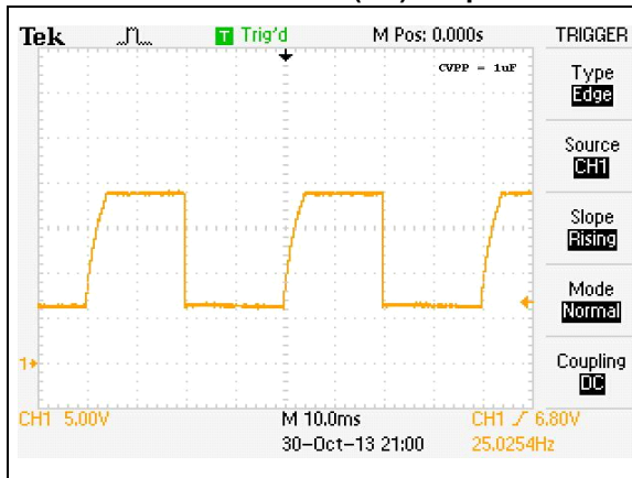
FIGURE 8-6: RIPPLE ON V_{PP} AND OUT00; V_{DD} = 3.3V , V_{PP} = 18V , CV_{PP} (C2) = 10 \mu F
