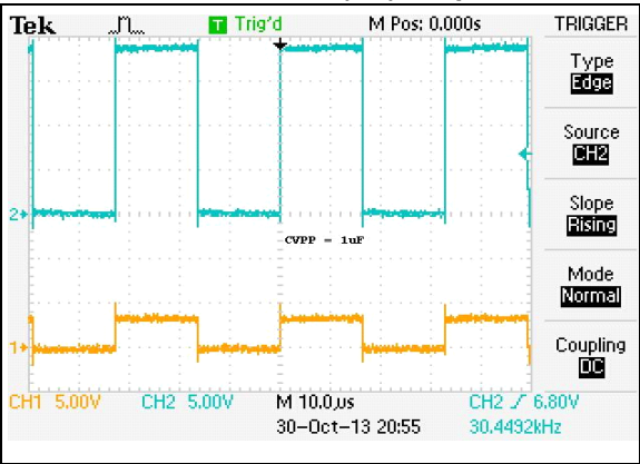
FIGURE 8-3: OE vs. OUT00; V_{DD} = 3.3V , V_{PP} = 18V , CV_{PP}(C2) = 1 \mu F
