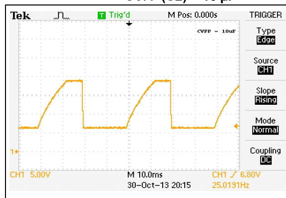
FIGURE 8-4: BOOST V_{\text{PP}} 6V TO 18V AND DISCHARGE 18V TO 6V; DISCHARGE ON, V_{\text{DD}} = 3.3\text{V} , \text{CVPP}(\text{C2}) = 10\text{ }\mu\text{F}
