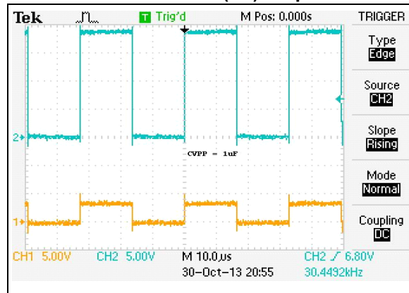
FIGURE 8-3: OE vs. OUT00; V_{\text{DD}} = 3.3\text{V} , V_{\text{PP}} = 18\text{V} , \text{CVPP}(\text{C2}) = 1\text{ }\mu\text{F}
