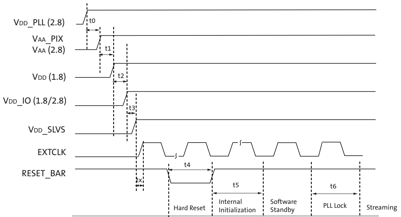
Figure 31: Power Up
