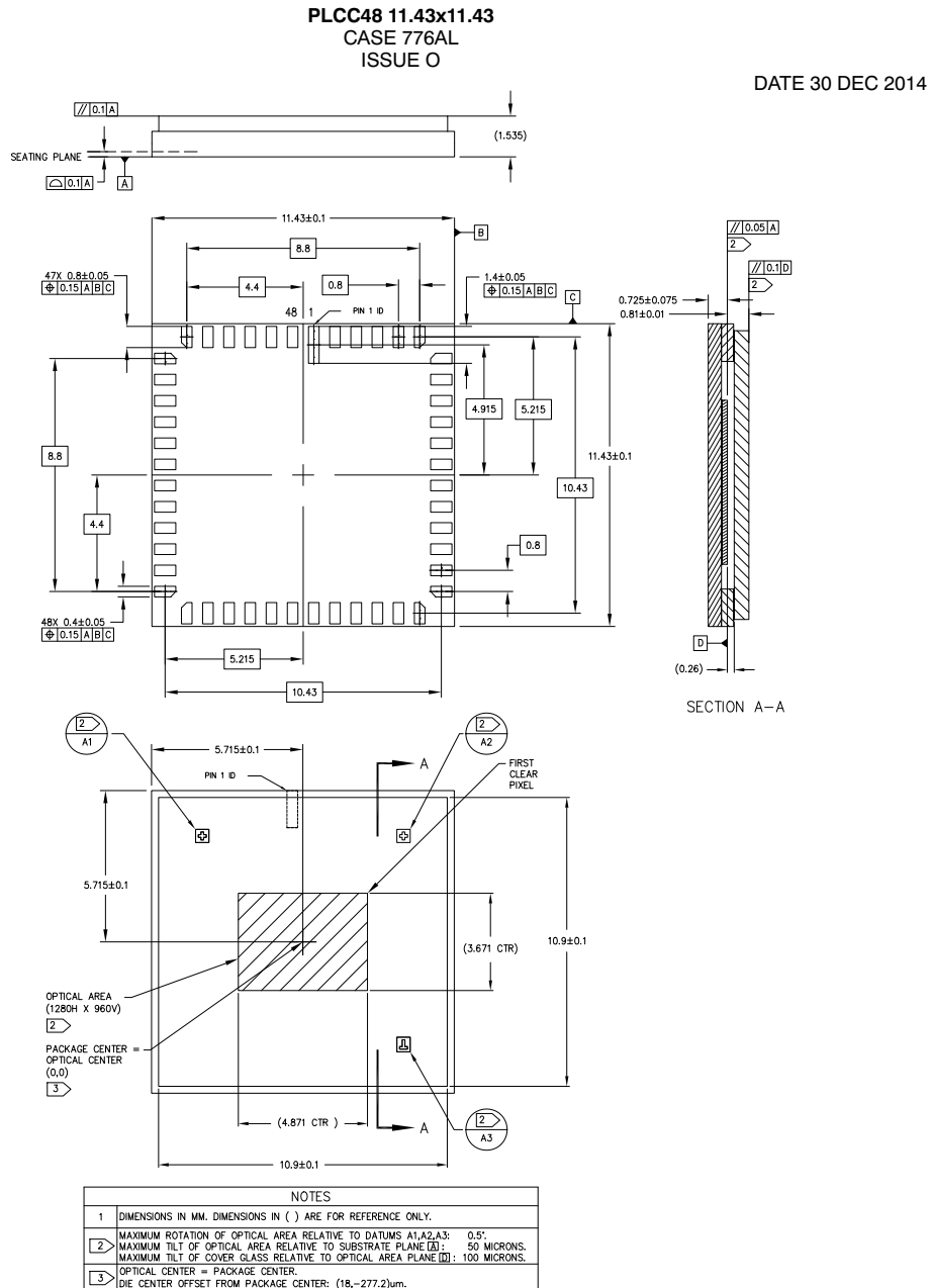
Figure 33: 48 PLCC Package Outline Drawing
