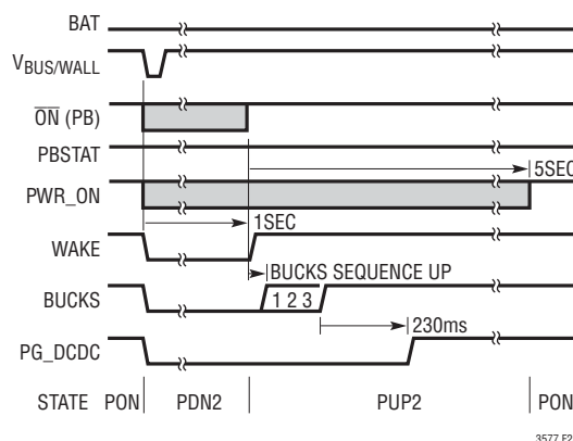
Figure 23. UVLO Minimum Off-Time
