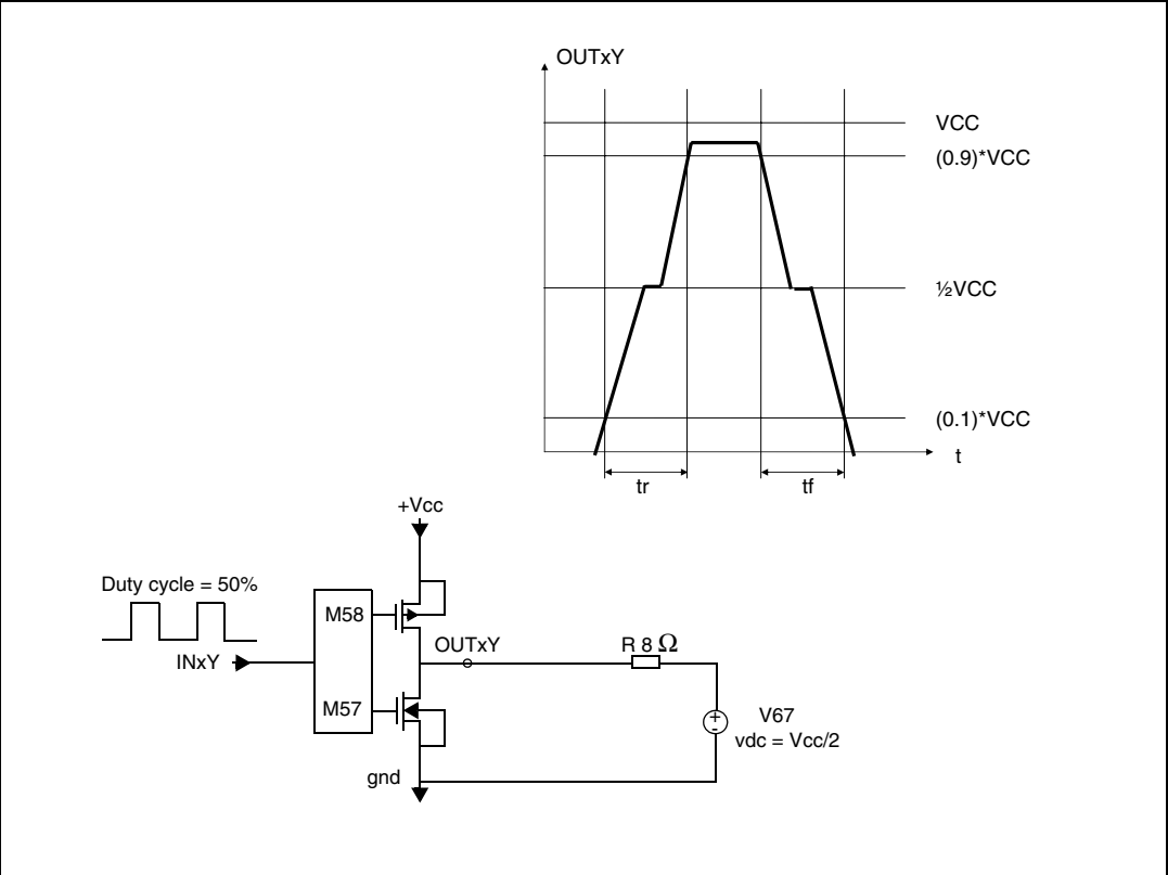
Figure 3. Test circuit
